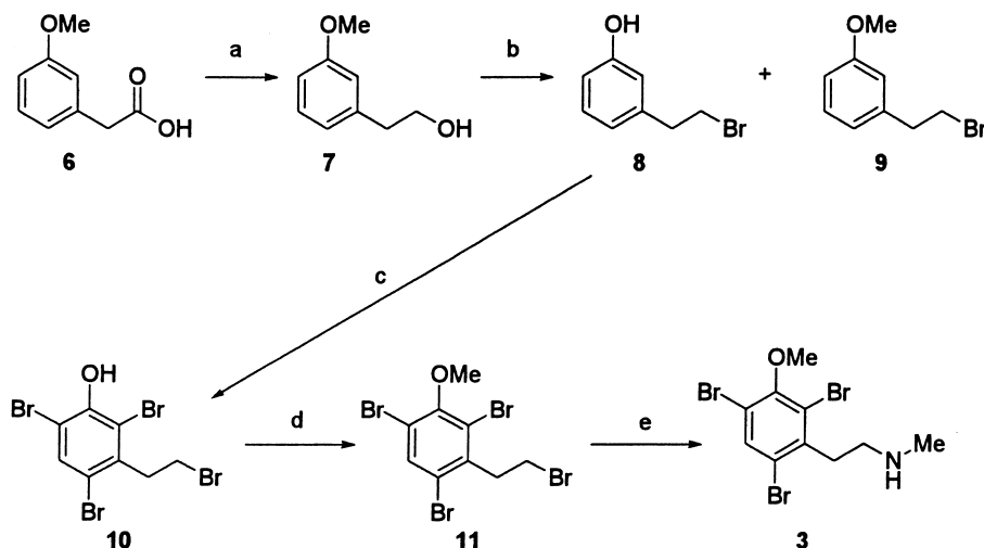
Scheme 1. Reagents and conditions: (a) LAH, THF, 87%; (b) 47% HBr, hexadecylPBr 3 Br, 8 76%, 9 5%; (c) Br 2 , AcOH, 82%; (d) CH 3 N 2 , MeOH, –5 °C, 82%; (e) 40% MeNH 2 , EtOH, 19%.
