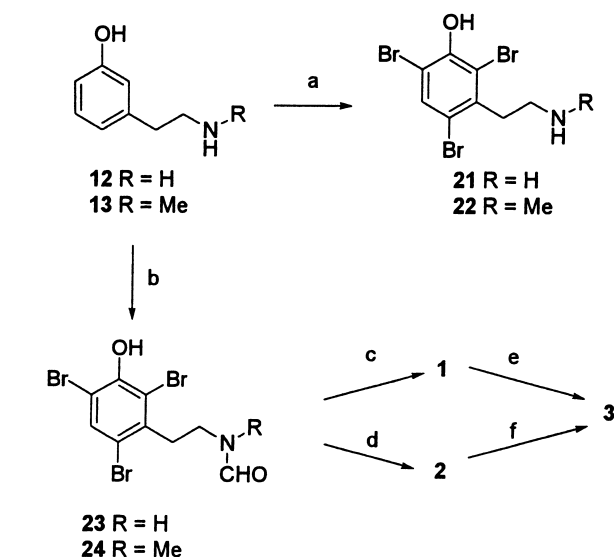
Scheme 5. Reagents and conditions: (a) \text{Br}_2 , HCl, AcOH, 21 71%, 22 54%; (b) i. \text{HCO}_2\text{Et} ; ii. \text{Br}_2 , AcOH, 23 97% (2 steps), 24 100% (2 steps); (c) \text{CH}_3\text{N}_2 , MeOH, -5^\circ\text{C} , 87%; (d) \text{CH}_3\text{N}_2 , MeOH, -5^\circ\text{C} , 95%; (e) \text{BH}_3 , THF, -5^\circ\text{C} , 67%; (f) 12 M HCl, MeOH, 74%.
