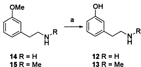
Scheme 2. Reagents and conditions: (a) 47% HBr, AcOH, 12 73%, 13 85%.
