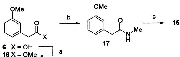
Scheme 3. Reagents and conditions: (a) HCl, MeOH, 91%; (b) 40% MeNH 2 , EtOH, 99%; (c) BH 3 , THF, 84%.
