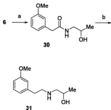
Scheme 7. Reagents and conditions: (a) 1-amino-2-propanol, (EtO) 2 -PO(CN), Et 3 N, THF, 61%; (b) BH 3 , THF, 82%.
