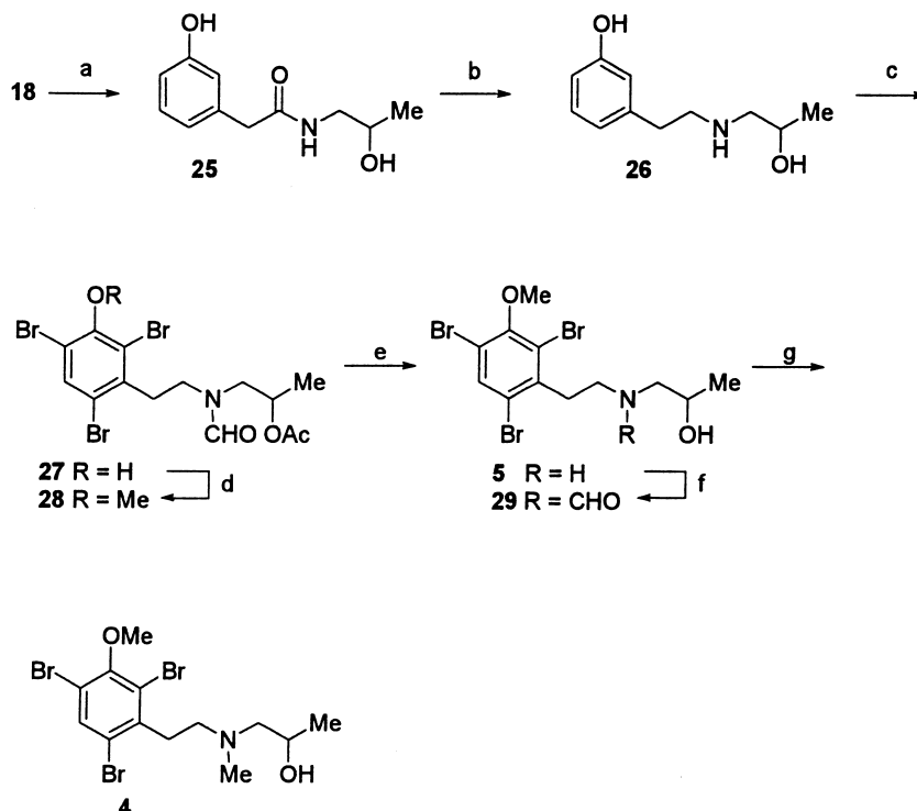
Scheme 6. Reagents and conditions: (a) 1-amino-2-propanol, (\text{EtO})_2\text{PO}(\text{CN}) , \text{Et}_3\text{N} , THF, -7 to -10^\circ\text{C} , 90%; (b) \text{BH}_3 , THF, 84%; (c) i. \text{HCO}_2\text{Et} ; ii. \text{Br}_2 , AcOH, 55% (2 steps); (d) \text{CH}_3\text{N}_2 , MeOH, 96%; (e) 12 M HCl, MeOH, 79%; (f) \text{HCO}_2\text{Et} , 96%; (g) \text{BH}_3 , thf, -5^\circ\text{C} , 71%.
